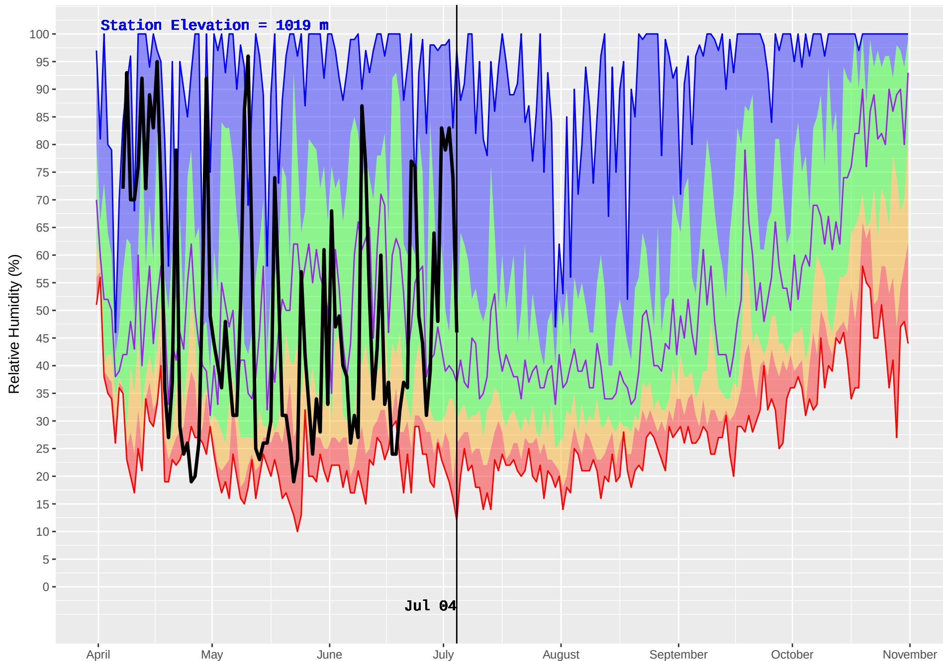
POWDER CREEK (380) : Historical (2001–2016) and Current (2018) Noon Relative Humidity
