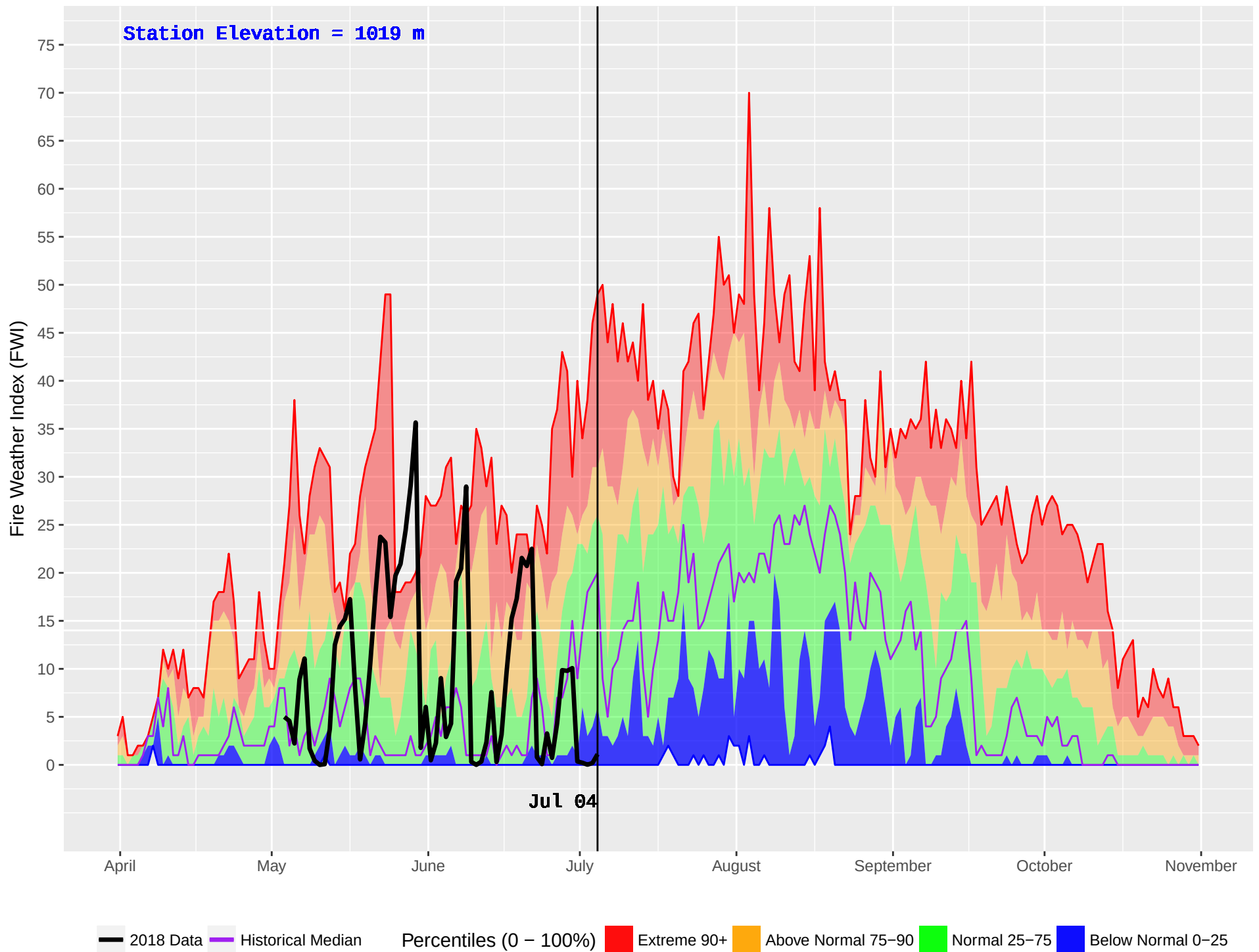
POWDER CREEK (380) : Historical (2001–2016) and Current (2018) Noon Fire Weather Index (FWI)
